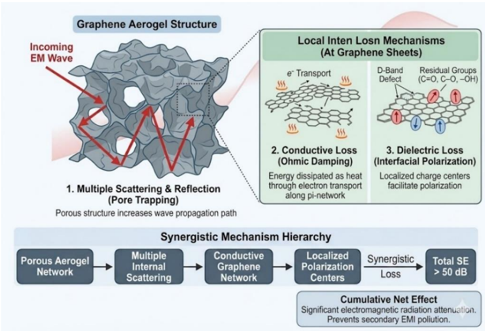
Figure 7: Diagrammatic representation of the synergy of electromagnetic interference shielding effects in camellia sinensis reduced graphene aerogel. The figure shows the hierarchy in the interaction between the macrostructure and microstructure for achieving high performance in the shielding effect.
