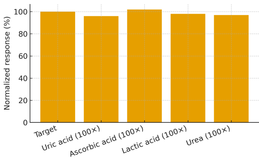
Figure 5. Selectivity: normalized signal (%) for target vs. common interferents (up to 100×).
