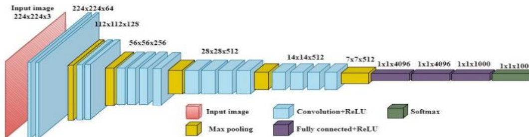
Architecture of VGG19
