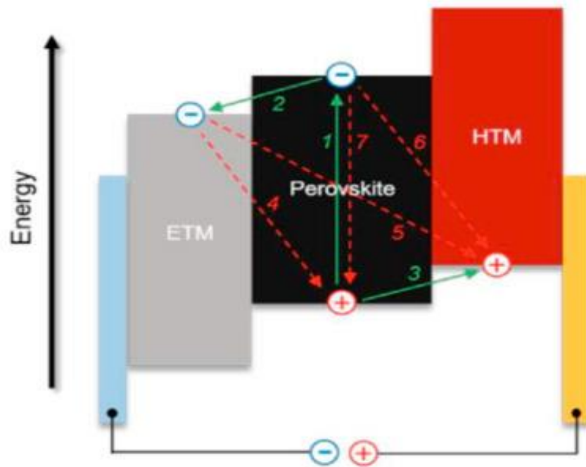
Figure 1: Perovskite photovoltaic compartments energy levels and charge-transfer mechanism [41].
