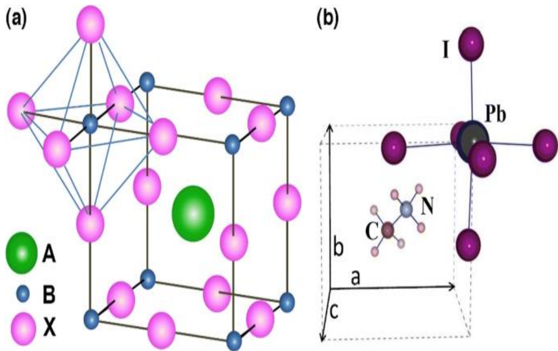
Figure 4: (a) Shows a larger ABX 3 perovskite structure in A cation occupying the cub octahedral site and BX 6 octahedral cation. (b) The cubic MAPbI 3 perovskite's unit cell [116].
