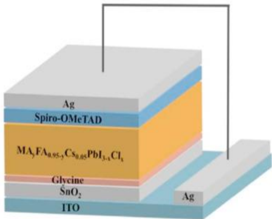
Figure 6: A schematic representation is provided for perovskite solar cells that utilize SnO 2 as their foundation [150].
