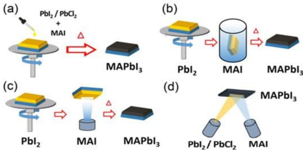
Figure 10: Methods for manufacturing perovskite solar cells are shown schematically. (a) One-phase procedure; (b) second stage process; (c) Method of Vapor-Sponsored result; (d) thermal vapour deposition technique. Amounts of precursors, wrapping reducing time, coating rotation time, and shifting speeds are fabrication-controlling factors for perovskite film quality or shape [233].
