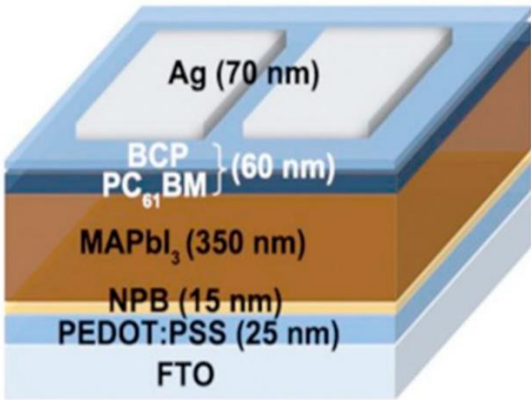
Figure 9: The structure of the NPB-based perovskite photovoltaic compartments device [232].
