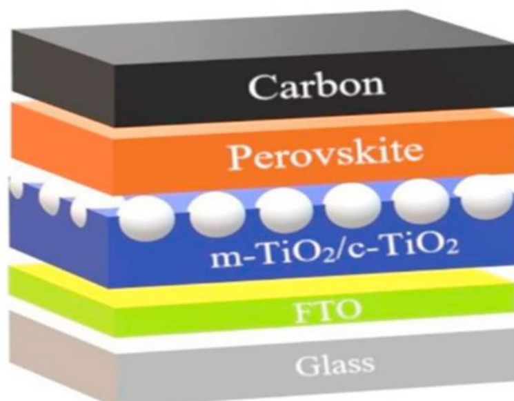
Figure 7: The image depicts a perovskite solar cell device PSC utilizing carbon-based CsPbBr 3 [174].
