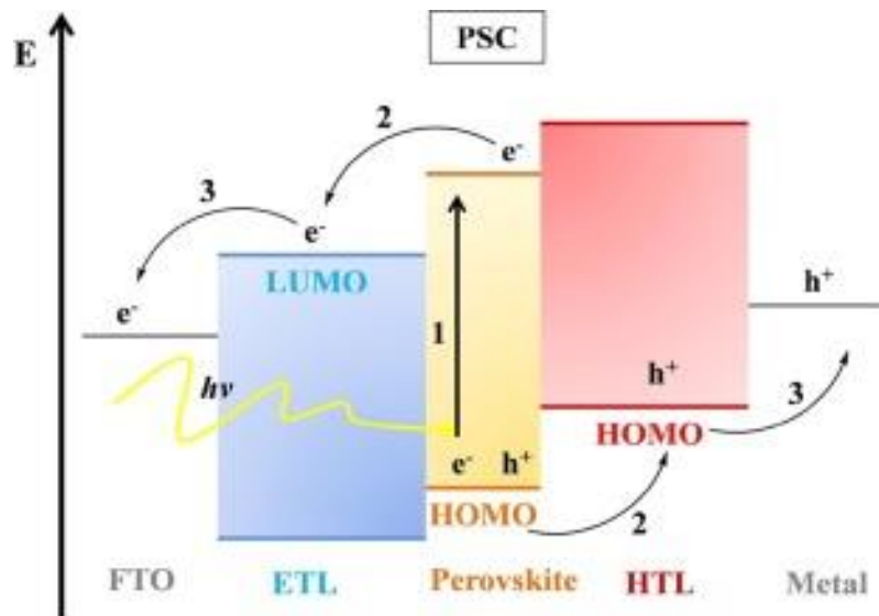
Figure 5: Show the Principles and working of PSCs [102].
