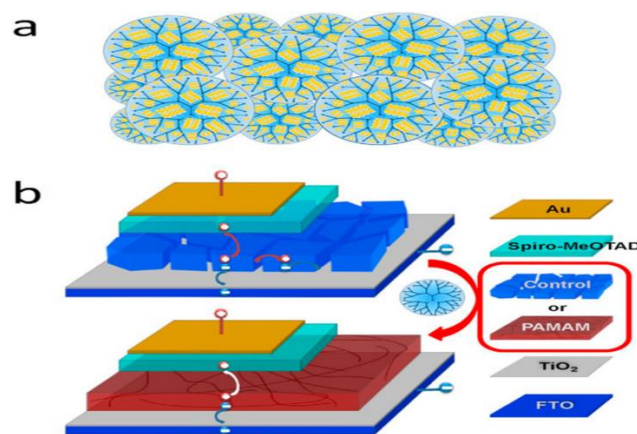
Figure 8: a) Diagrammatic illustration of PAMAM dendrimers controlling the structure of perovskite b) Device arrangement of regulator and PAMAM-adapted perovskite photovoltaic compartments [224].
