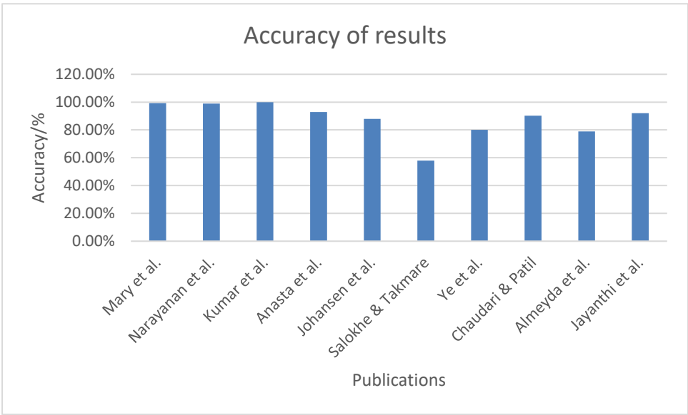
Figure 6: Accuracy Percentage of Ten Publications
