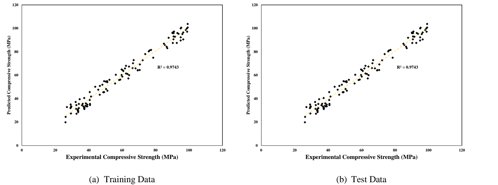
Figure 7: Plot of Predicted vs Experimental values for RF Model
