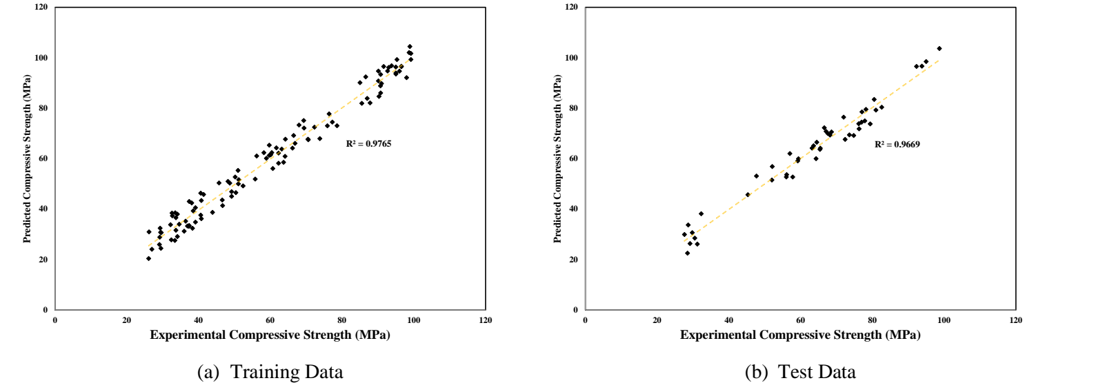
Figure 8: Plot of Predicted vs Experimental values for KNN Model
