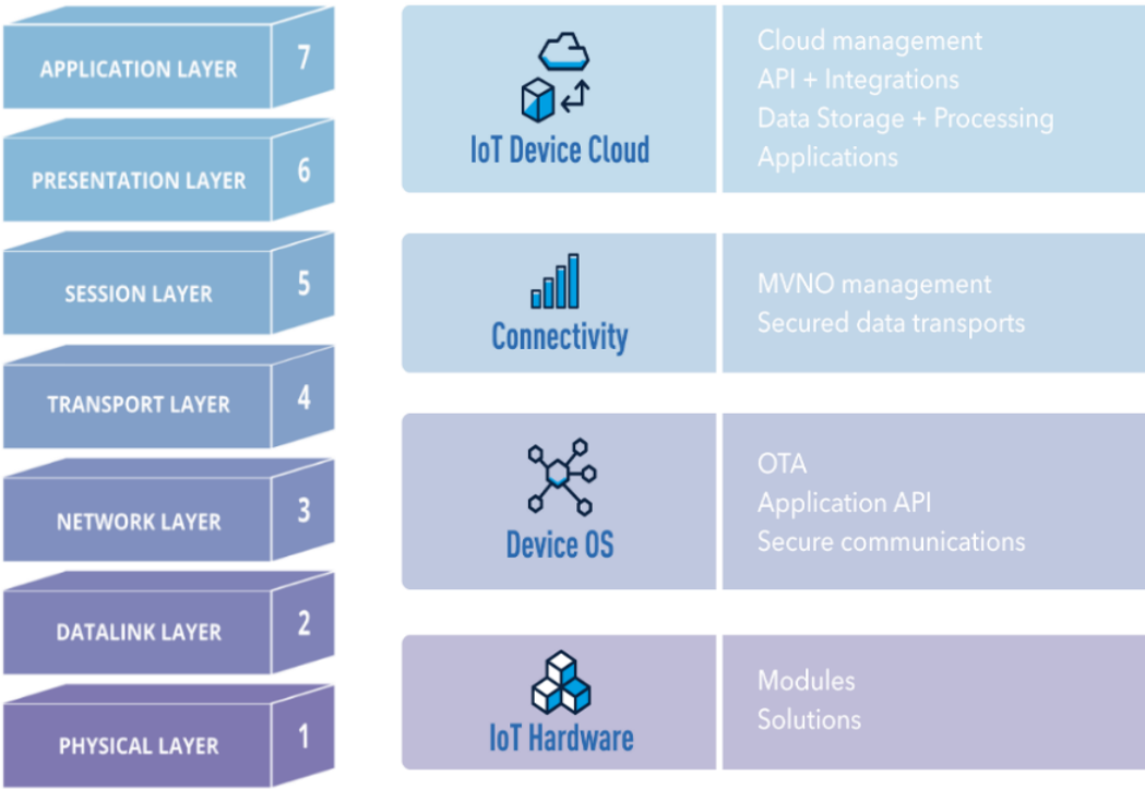
Figure 8: Stack protocol [30]
