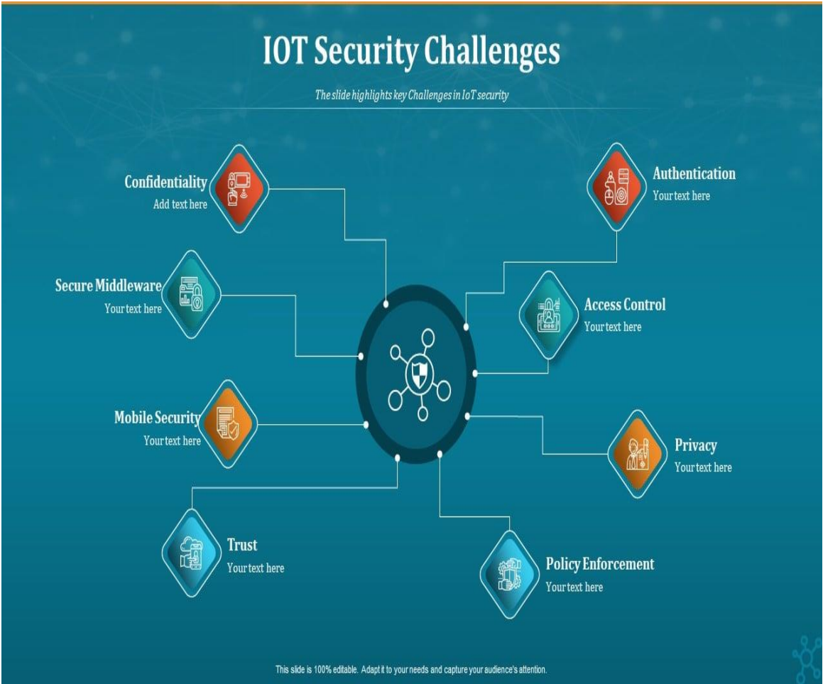
Figure 6: Security challenges [24]
