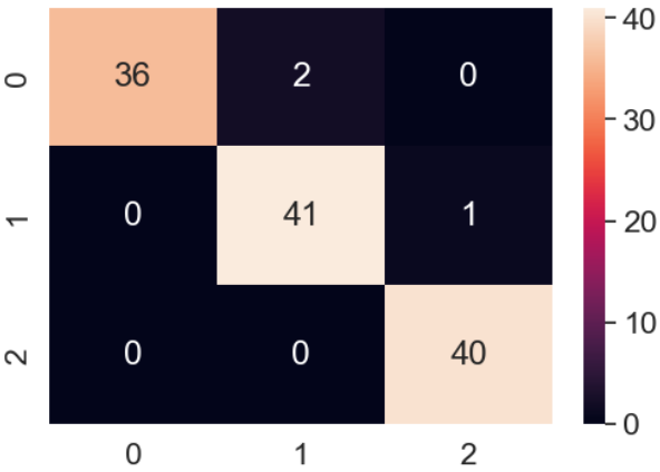
Figure 6: Confusion Matrix of MLP.
