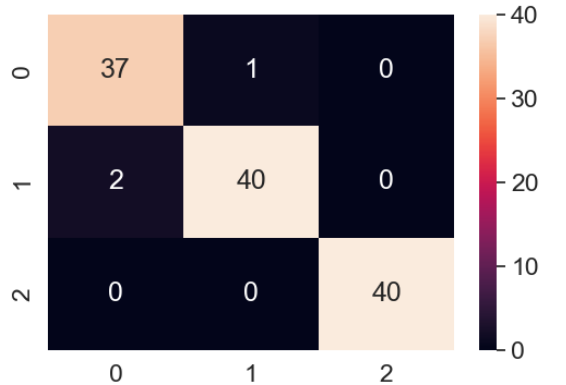
Figure Error! No text of specified style in document.: Confusion Matrix of RF.
