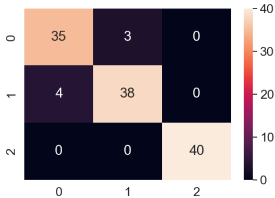
Figure 5: Confusion Matrix of SVM.
