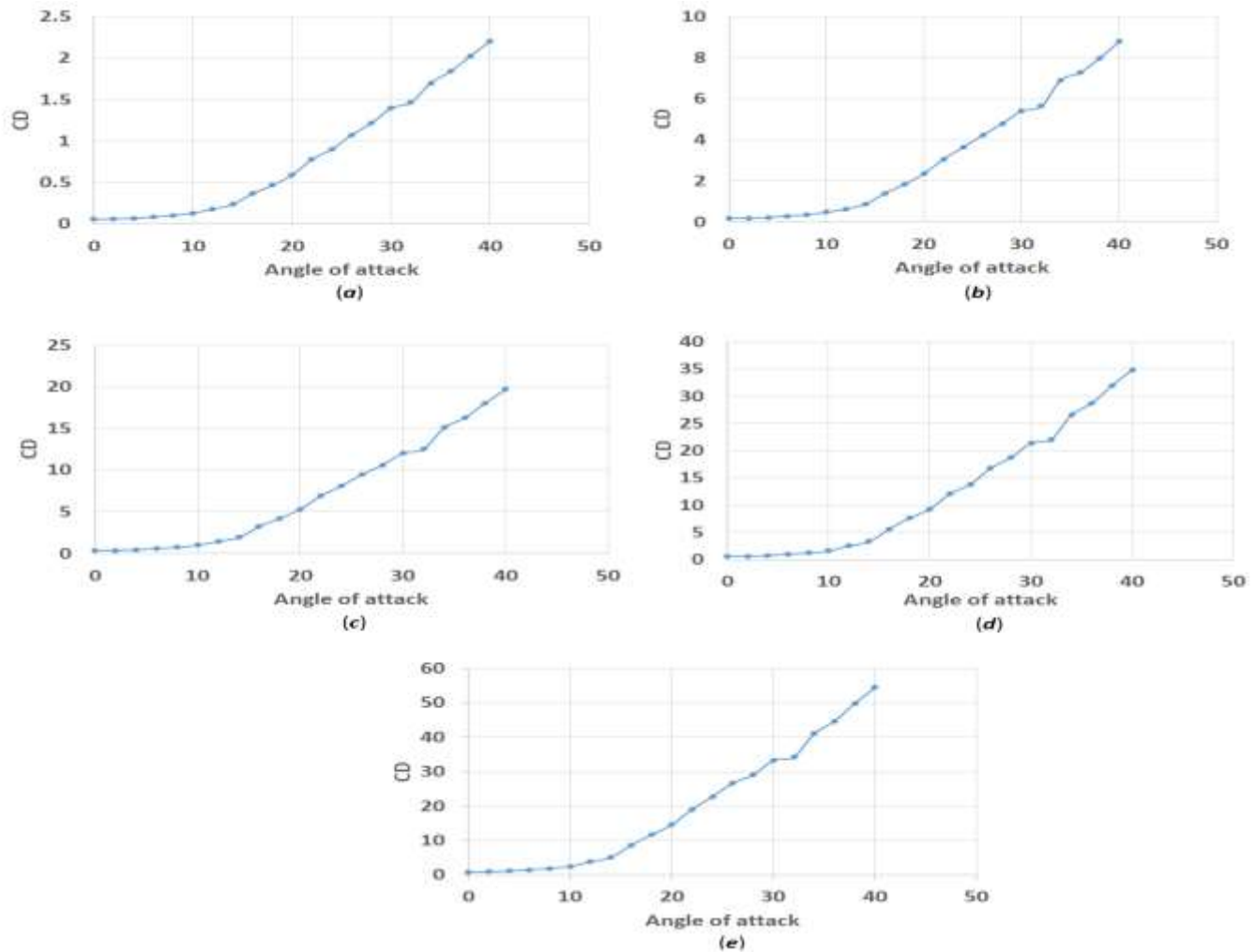
Fig. 5. Coefficient of drag C_D against \alpha for inlet velocity (a) u = 2 m/s, (b) u = 4 m/s, (c) u = 6 m/s, (d) u = 8 m/s and (e) u = 10 m/s
