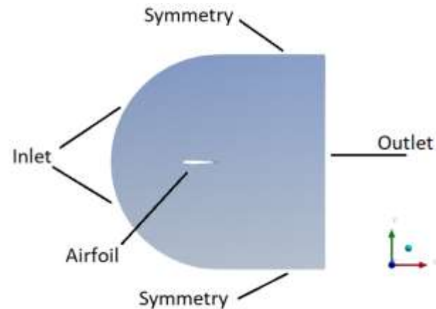
Fig. 2. Computational domain
