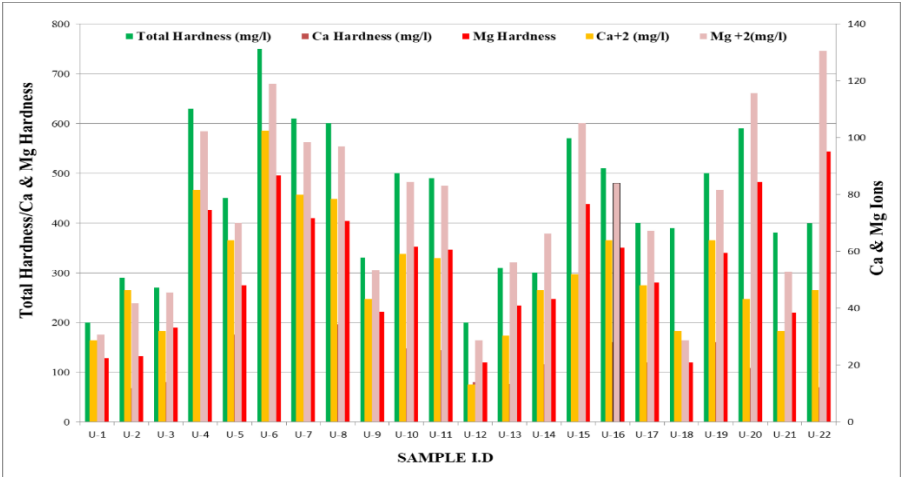
Figure 3. Total Hardness, Calcium Hardness/Magnesium Hardness & Calcium/ Magnesium Ions in Water Samples
